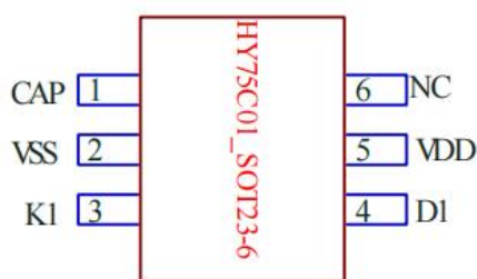
HY75C01 SOT-23-6
